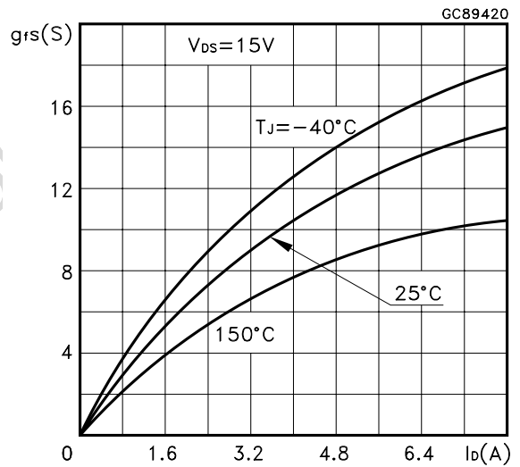
Transconductance n-ch
